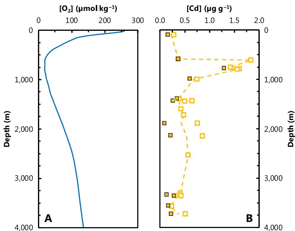
Figure 18. Cadmium concentrations in California Margin sediments. (a) Regionally representative [O_2] profile from the Northeast Pacific showing broad minimum between 600–800 m. Profile from 35.5^\circ N , 122.5^\circ W (from World Ocean Atlas; Garcia et al., 2014). (b) Solid phase Cd concentration data from van Geen et al. (1995) for Northeast Pacific coretop (closed symbols) and “slightly deeper” (8–10 cm; open symbols) sediment samples; dashed line indicates arithmetic mean. These samples evidence a maximum in authigenic Cd deposition at the top of the oxygen minimum zone (OMZ), which may originate from processes occurring in the water or sediment column.
